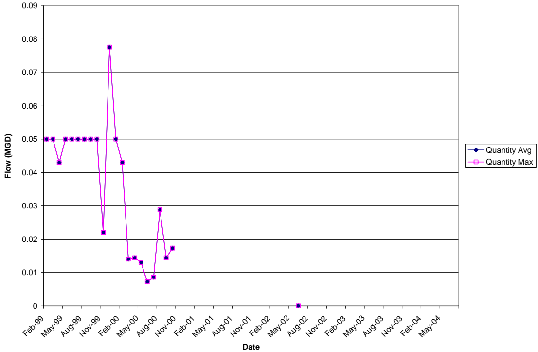
Figure A-8: Norfolk Southern Railway Co - East End Shops (VA0001511 Outfall 3) Average and Maximum Monthly Flow
