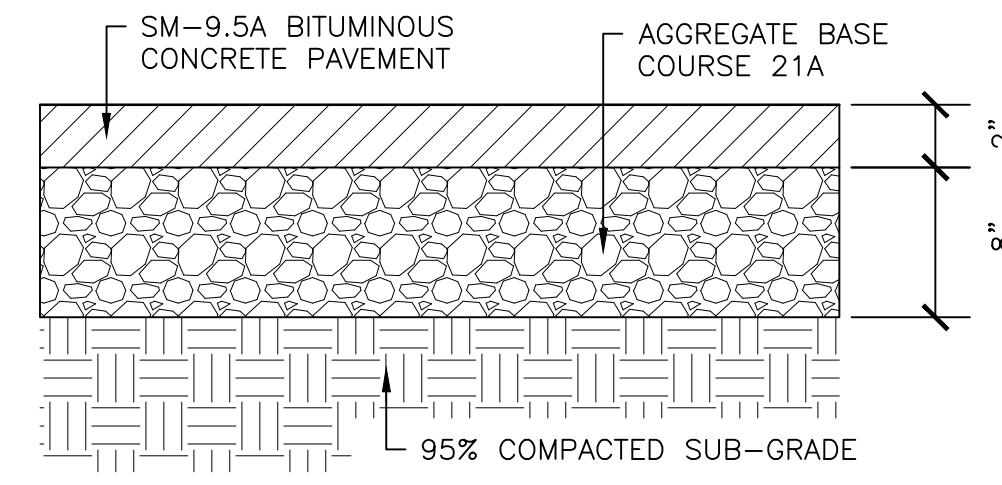
LIGHT DUTY PAVING - DETAIL NTS
