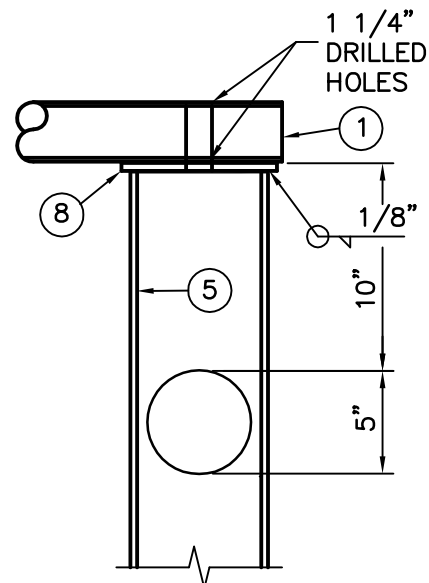
END POST DETAIL
