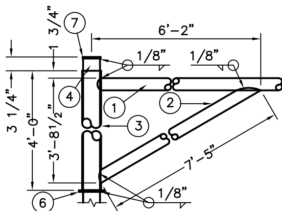
HINGE DETAIL
