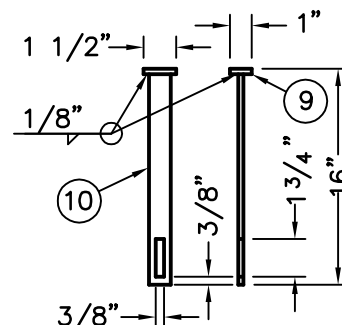
LOCKING PIN
