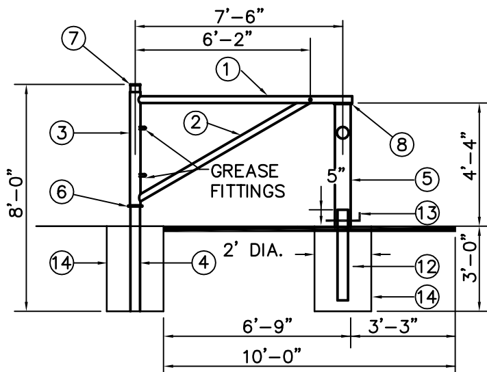
GATE
