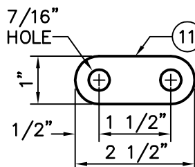
LOCKING BAR
