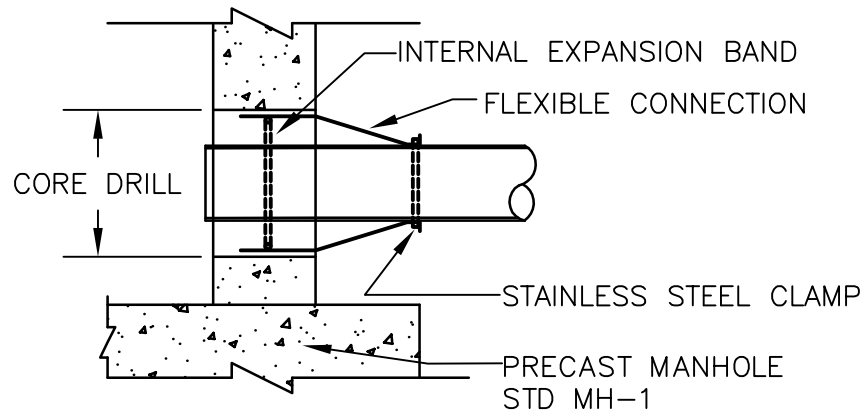
ENLARGED SECTION
