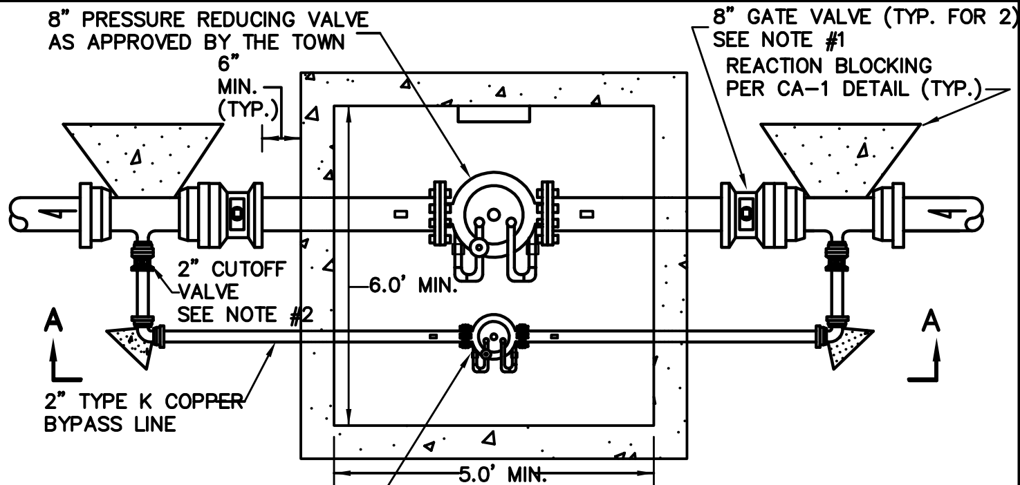
PLAN
