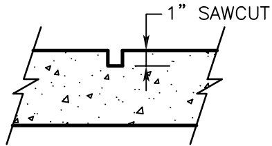
CONTROL JOINT DETAIL
