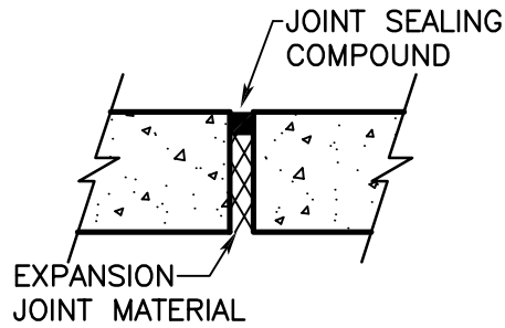
EXPANSION/CONSTRUCTION JOINT DETAIL
